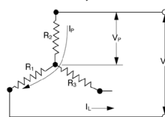
3-Phase Wye (Balanced Load)
